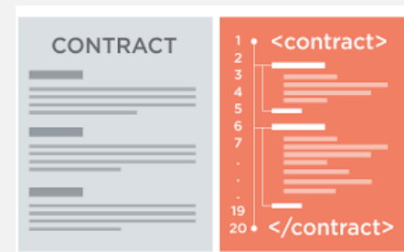
Smart contract
